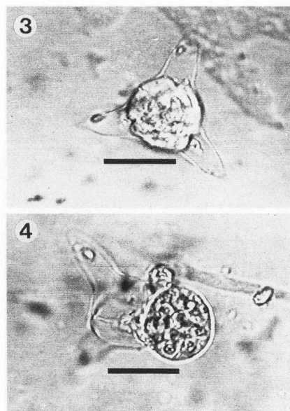
Figs. 3–4. Waterborne aurantiactinospore of Thelohanelius nikolskii released into the water 124 days post infection. Fig. 4. showing discharge of sporoplasm. Digitized video image. Bar = 20 µm
