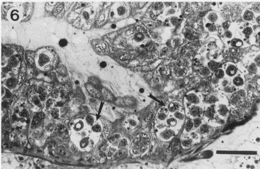
Figs. 5–6. Semithin section of Branchiura sowerbyi infected with Thelohanellus hovorkai mature actinospores (101 days post infection). Fig. 5: Arrows indicate aurantiactinospores of T. hovorkai developing in the gut epithelium. Bar = 200 µm Fig. 6: Higher magnification of the gut epithelium. Arrows indicate well-discernible polar capsules. Bar = 80 µm
