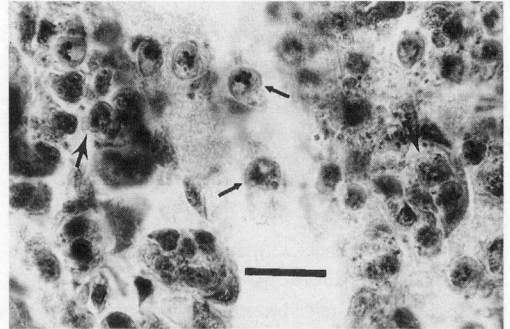
Fig. 7. Histological section of the gut of an experimentally infected Branchiura sowerbyi . Large arrows indicate pansporocysts containing mature aurantiactinospores of Thelohanellus hovorkai in the gut epithelium. Small arrows indicate free aurantiactinospores of T. hovorkai released from the intestinal epithelium into the lumen. The episporic and some of the caudal processes are well discernible. Stained with haematoxylin and eosin. Bar = 60 µm
