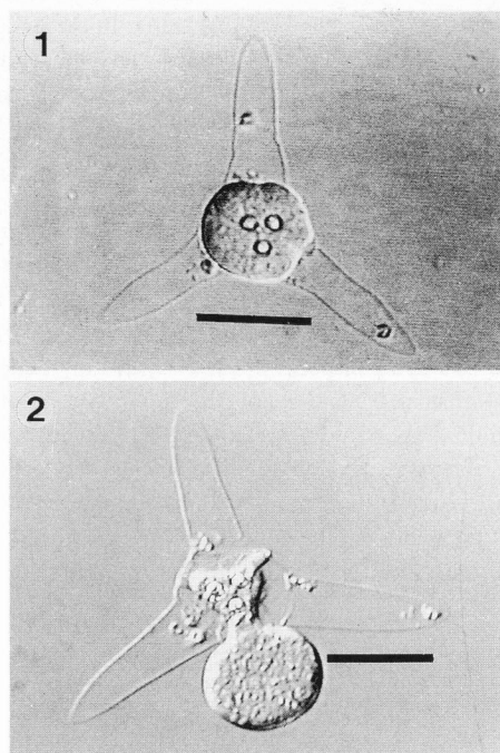
Figs. 1–2. Waterborne aurantiactinospore of Thelohanelius hovorkai floating in the water 104 days post infection. Fig. 2. showing discharge of sporoplasm. Digitized video image. Bar = 20 µm
