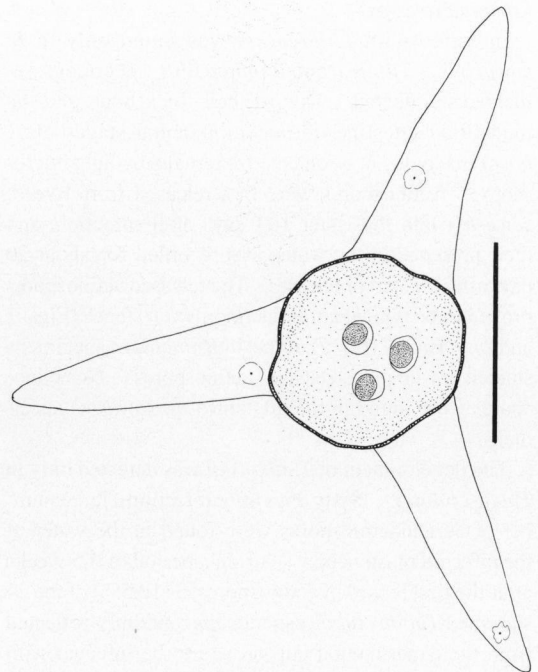
Fig. 8. Schematic illustration of the aurantiactinomyxon spore of Thelohanellus hovorkai . Bar = 20 µm.
