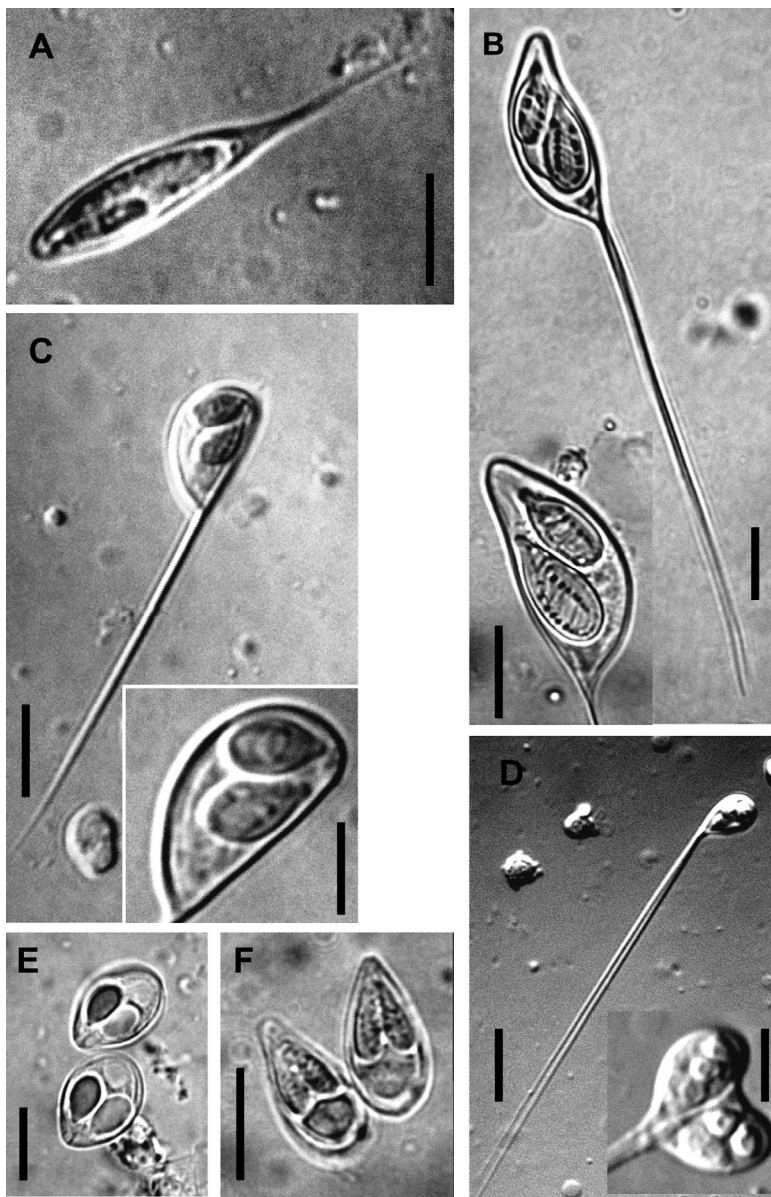
Fig. 2. Hennegouya , Hennegoides and Myxobolus spp. spores found in Pangasius hypophthalmus . (A) Hennegouya shariffi sp. n. Scale bar = 5 \mu m. (B) Hennegoides pangasii sp. n. Scale bar = 10 \mu m (inset: spore body of H. pangasii sp. n. Scale bar = 10 \mu m). (C) Hennegoides malayensis sp. n. Scale bar = 10 \mu m (inset: spore body of H. malayensis sp. n. Scale bar = 5 \mu m). (D) Hennegoides berlandi sp. n. Scale bar = 10 \mu m (inset: still attached developing spore bodies of H. berlandi sp. n. Scale bar = 5 \mu m). (E) Fixed spores of M. baskai sp. n. without caudal appendages. Scale bar = 10 \mu m. (F) M. pangasii sp. n. Scale bar = 10 \mu m
