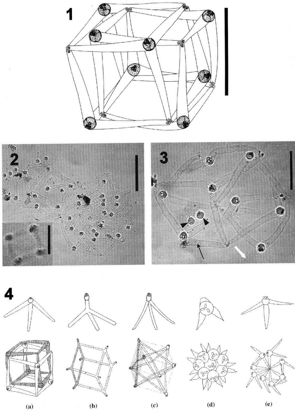
Figures 1-4. 1. Diagrammatic illustration of the hungactinomyxon spore complex. 2. Mass of unseparated double-cubes of hungactinomyxons. Free spores of guyenotia are also apparent. Inset: a regular double-cube of a hungactinomyxon, apical view. 3. A freshly released hungactinomyxon floating in water and composed of echinactinomyxon units with united caudal processes. One process (white arrow) of an echinactinomyxon unit torn from the junction (arrow). Two guyenotia actinospores are found inside the grid (arrowheads). 4. Diagrammatic illustration of reticulated actinosporean collective groups: hungactinomyxon (a), siedleckiella (b), antonactinomyxon (c) and two synactinomyxon (d, e) types (lower row) and their actinospore unit (upper row); drawings not to scale. Scale-bars: 100 \mu\text{m} .
