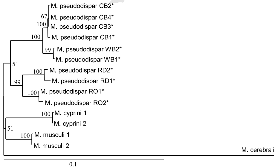
Figure 3 Phylogenetic tree generated by distance matrix analysis and showing relationships between Myxobolus spp. collected from the muscle of cyprinid species. The length of the edited alignment sequences was 972 bp, containing a 511-bp fragment from the 5'-end of the 18S rRNA gene and a 461-bp fragment from the 3'-end. Myxobolus cerebralis (U96492) was chosen as an outgroup. Sequences published in this study are listed in Table 2. Numbers at nodes indicate bootstrap confidence levels obtained by distance matrix analysis. Scale bar is equal to 10% difference. *CB: common bream, WB: white bream, RO: roach, RD: rudd.
