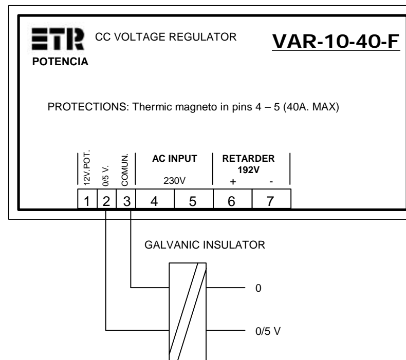
CONTROL BY VOLTAGE WITH GALVANIC INSULATION
